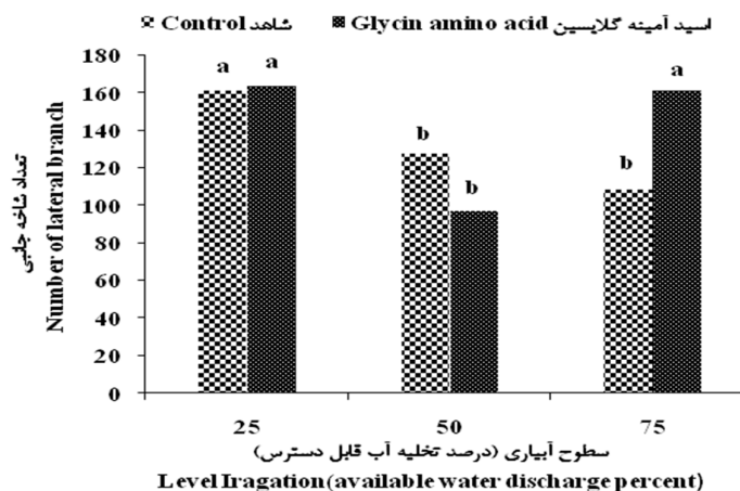
Fig. 2. Interaction effects of irrigation treatments and foliar application type on hyssop plant ( Hyssopus officinalis L.) number of lateral branch.
