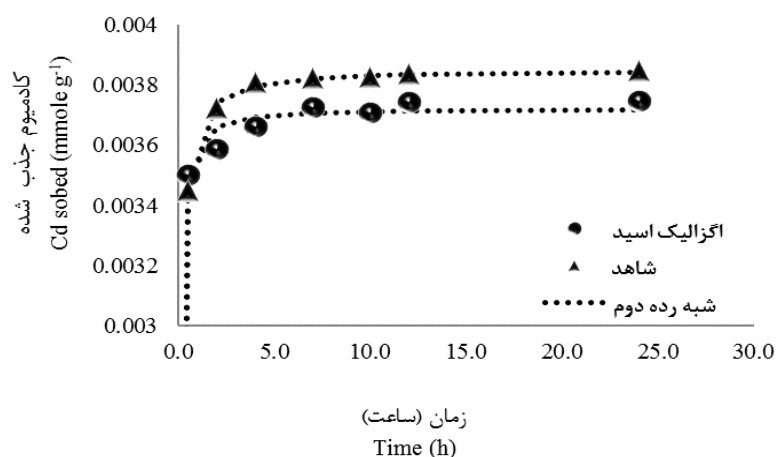
Figure 4. Goodness of pseudo-second- order equation on time-dependent sorption of Cd onto clay fraction of soil.
