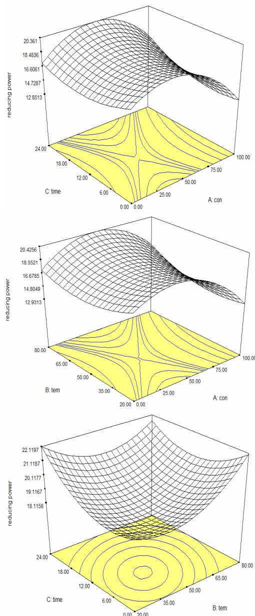
Fig 2 Three-dimensional diagram of changes in the reducing power amount of Ajowan seed ethanolic extracts under different conditions. a; ethanolic extract concentration and extraction time (extraction temperature= 50), b; ethanolic extract concentration and extraction temperature (extraction time= 12 hours), c; extraction time and temperature (ethanolic extract concentration= 50%)
