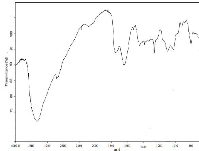
Fig 3 FTIR spectrum of pectin extracted from pumpkin cap in acidic conditions ranging from 400 to 4000 centimeters -1
