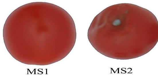
Fig 5 Two ripening stages MS1 and MS2 derived for cherry tomatoes.
