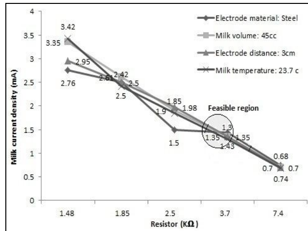
Fig 7 Chart of Changes in the electrical current density in terms of the circuit resistor with a steel electrode, with equal cell coefficient 3 \text{ (cm}^{-1}\text{)} at 23.7^\circ \text{C} , for two minutes and 45 cc milk.
