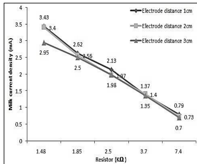
Fig 5 chart of Changes in the electrical current density of milk in terms of the circuit resistor at intervals of 1, 2 and 3 cm between steel electrodes at 20.7 ° C with 25 cc of milk.
