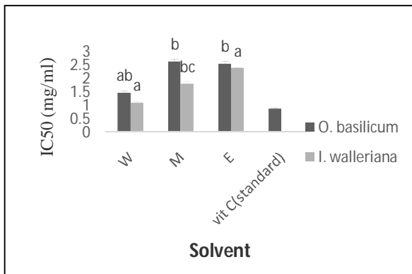
Fig 2 Antioxidant properties (IC50) of Ocimum basilicum and Impatiens walleriana extracts (Water: W, Methanol: M, Ethanol: E) using water bath method. The values with different superscript letters in a column are significantly different ( p < 0.05 ).
