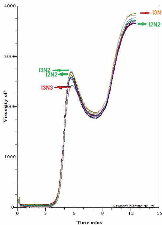
Fig 2 The viscosity curve of Gilaneh rice variety in interaction between irrigation and nitrogen treatments
