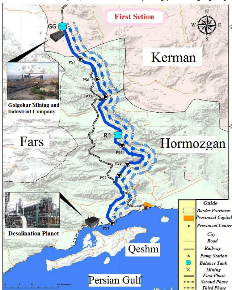
Fig. 3- Water supply from Persian Gulf- first section
