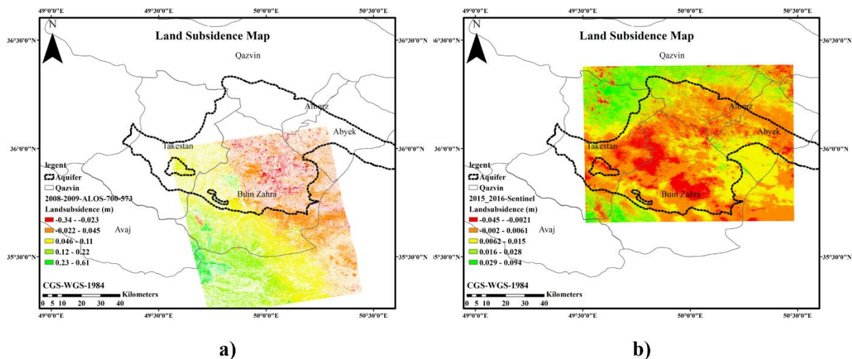
Fig. 10- Land subsidence map in Qazvin aquifer for the period of a) 2008-2009 and b) 2015-2016
