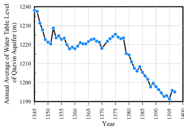
Fig. 11- The groundwater table variations of Qazvin aquifer for the period of 1966-2018
