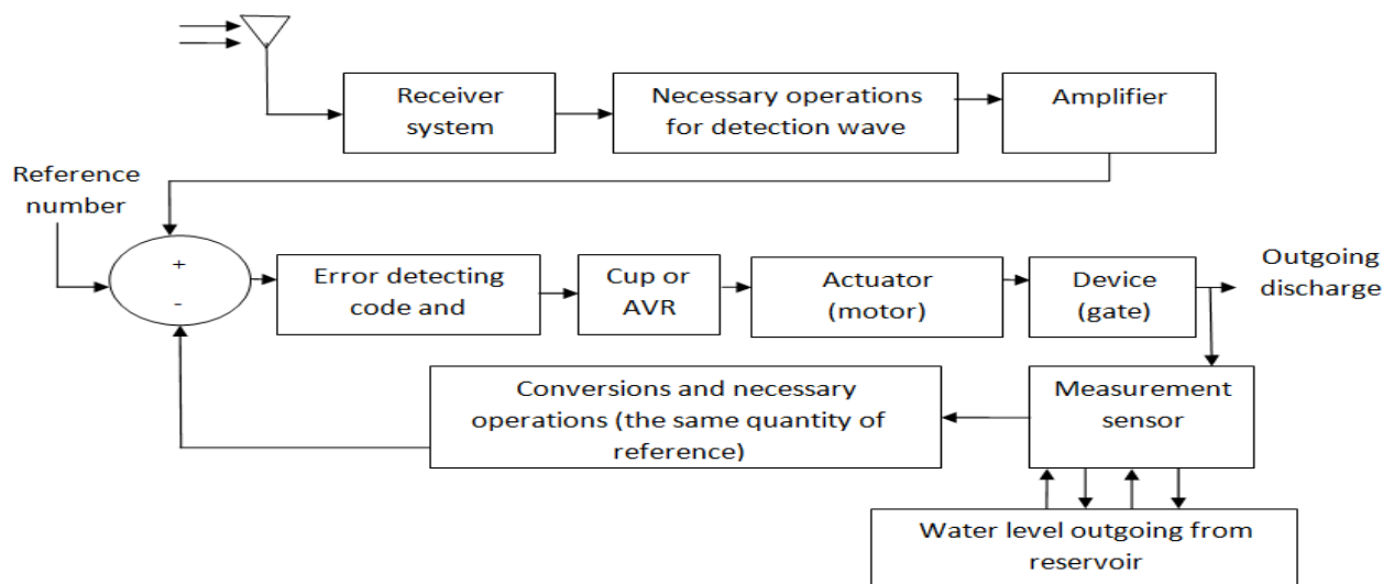
Fig. 5- Receiver, water height analyzer, gate control system
