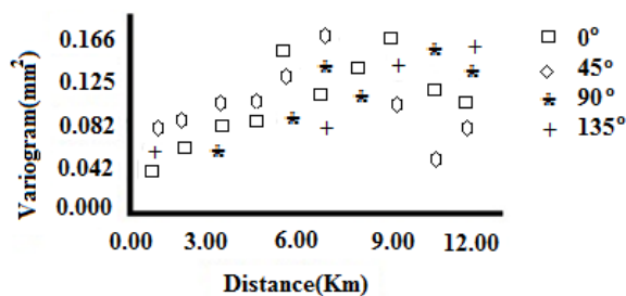
Fig 2 - Directional semivariogram for July evapotranspiration
