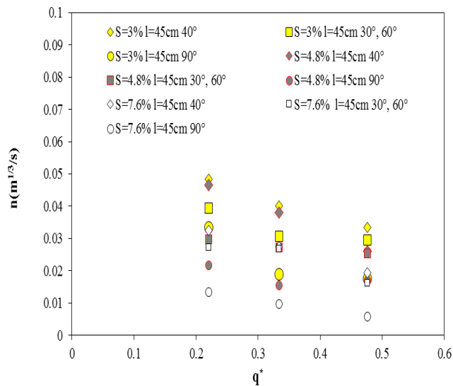
Fig. 4- Manning roughness coefficient variations versus dimensionless flow rate tested at relative spacing of A) 0.6; B) 1.2; C) 1.8
