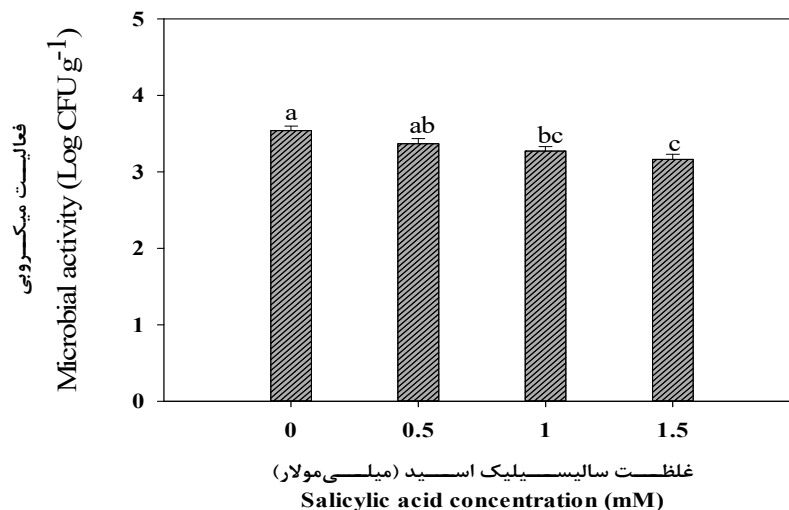
Fig 4. Effect of salicylic acid on microbial activity of kiwifruit cv. Hayward after 14 weeks storage at 1.5±1 °C for 14 weeks storage. Mean values in each column followed by the same letters are not significantly different ( P < 0.05 ).
