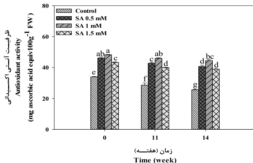
Fig 3. Effect of salicylic acid on antioxidant activity of kiwifruit cv. Hayward at 1.5±1 °C for 14 weeks storage. Mean values in each column followed by the same letters are not significantly different ( P < 0.05 ).
