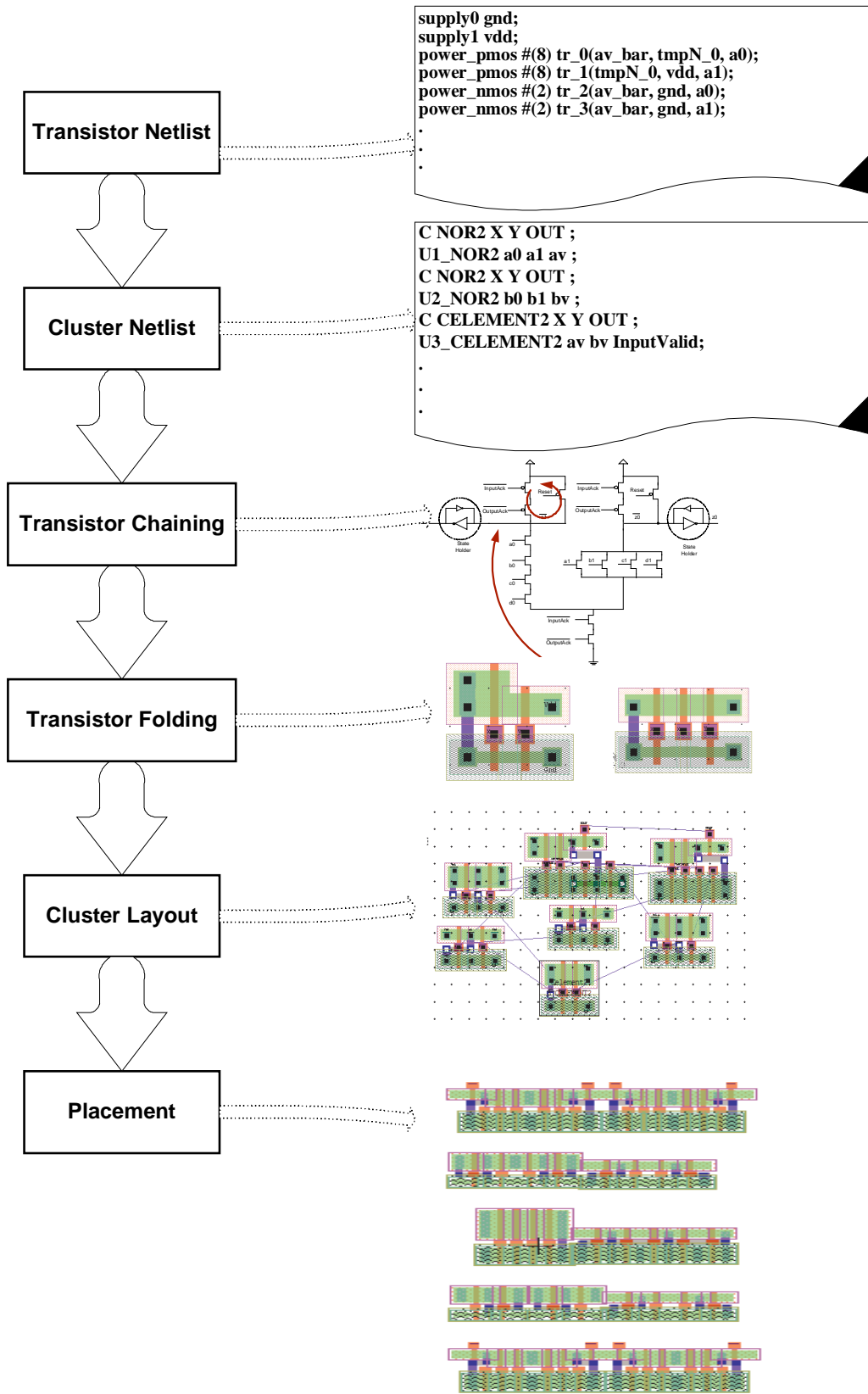
Figure2. Design flow
