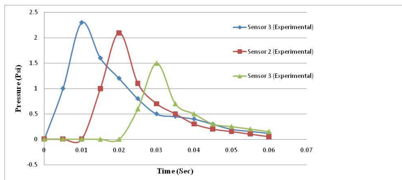
Figure 7: Pressure distribution in comparison the time during the experimental tests for different points
