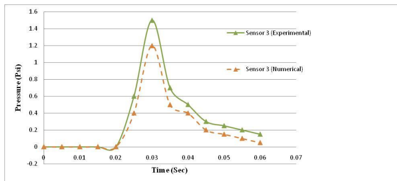
Figure 10: Comparison of results of numerical simulation and experimental test for pressure sensor no. 3
