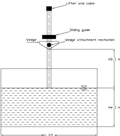
Figure 4: Illustration of test set-up's main elements and basic dimensions
