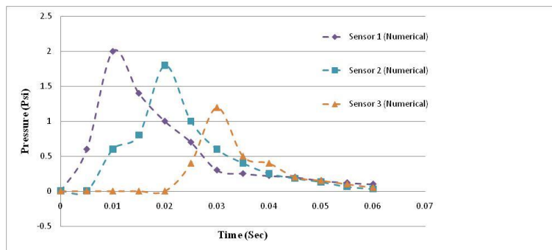
Figure 6: Pressure distribution in comparison the time during the numerical analysis for different points
