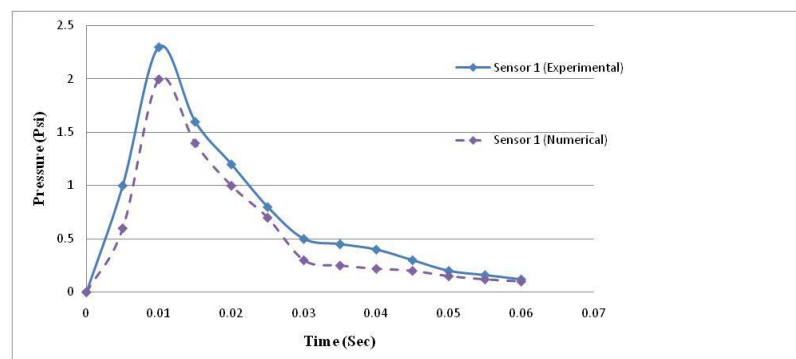
Figure 8: Comparison of results of numerical simulation and experimental test for pressure sensor no. 1
