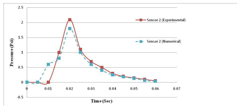
Figure 9: Comparison of results of numerical simulation and experimental test for pressure sensor no. 2
