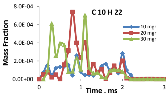
Figure 6. Mean diesel mass fraction versus time for porosity 90 % and different injected fuel
