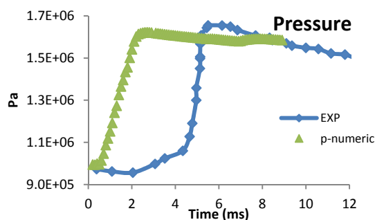
Figure 3. comparison CFD results with experimental data
