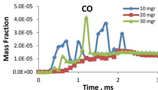
Figure 7. Mean Carbon monoxide mass fraction versus time for porosity 90 % and different injected fuel
