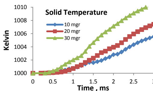
Figure 11. Mean solid phase temperature versus time for porosity 90 % and different injected fuel
