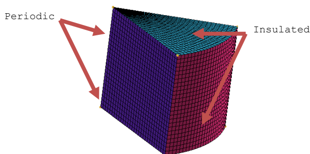
Figure 2. Computational mesh for the PM chamber
