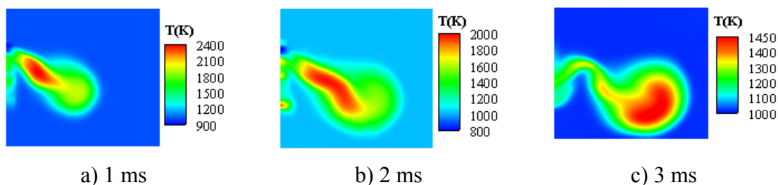
Fig 4. Fluid temperature in free volume
