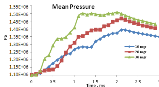
Figure 9. Mean pressure versus time for porosity 90 % and different injected fuel
