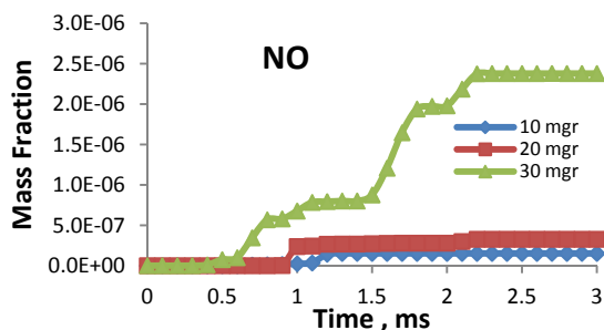
Figure 8. Mean nitrogen monoxide mass fraction versus time for porosity 90 % and different injected fuel
