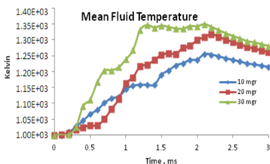
Figure 10. Mean fluid phase temperature versus time for porosity 90 % and different injected fuel
