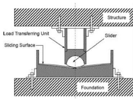
Figure 1. Details of the VFPI [20].
