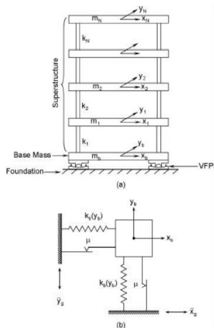
Figure 2. Modeling of multi-story building and the VFPI.
