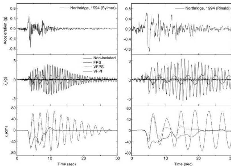
Figure 5. Time variation of top floor absolute acceleration and isolator displacement of five-story building isolated with the FPS ( T_b=2.0 sec and \mu=0.02 ), VFPS ( T_b=2.0 sec, T_y=1.5 sec and \mu_{max}=0.15 ) and VFPI ( T_b=2.0 sec and \mu=0.02 ) under Northridge, 1994 (Sylmar) and Northridge, 1994 (Rinaldi) near-fault ground motions.
