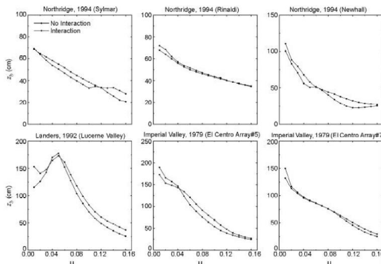
Figure 14. Comparison of isolator displacement of five-story building isolated by the VFPI during various near-fault ground motions (considering with and without interaction).
