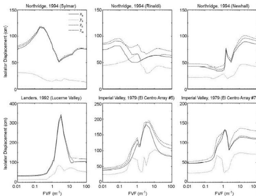
Figure 8. Variation of the peak isolator displacements, x_b , y_b , z_b , and z_m , of five-story building isolated with the VFPI against the FVF for various near-fault ground motions.
