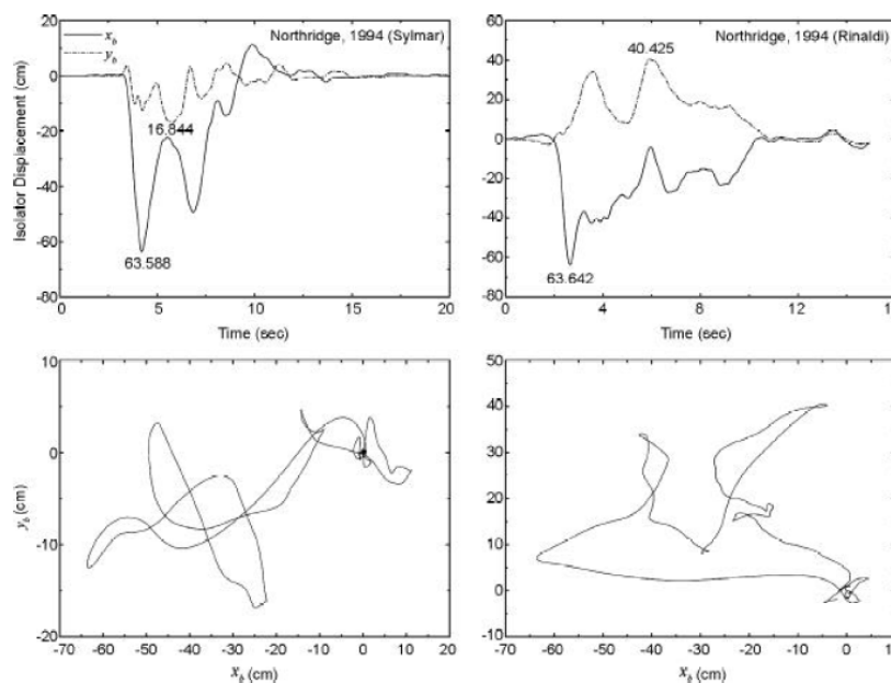
Figure 7. Top: Time variation of x_b and y_b of five-story building isolated with VFPI ( T_f = 2.0 sec and \mu = 0.02 ) under different near-fault ground motions. Bottom: Correlation between x_b and y_b .
