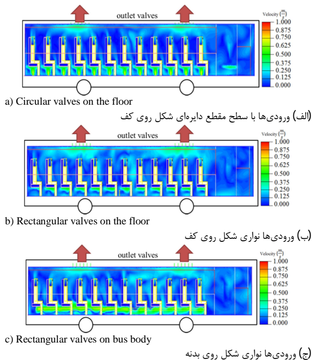
Fig. 5 Speed contours for three cases inlet
