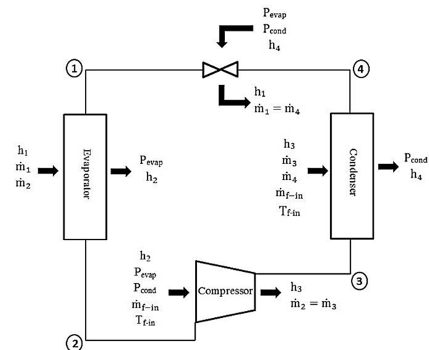
Fig.5 Essential inputs and outputs for components model in a coupled system
