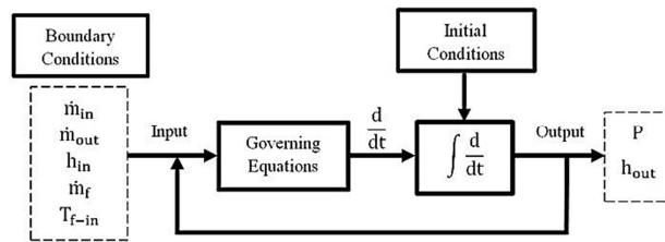
Fig.3 Solution algorithm in moving boundary method
