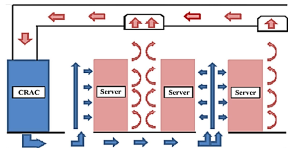
Fig. 1 Schematic of a data center [6]
