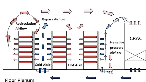
Fig. 2 Recirculation and bypass airflow in a data center [1]
