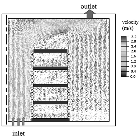
Fig. 7 velocity vectors for v_{in} = 1.2 (m/s)
