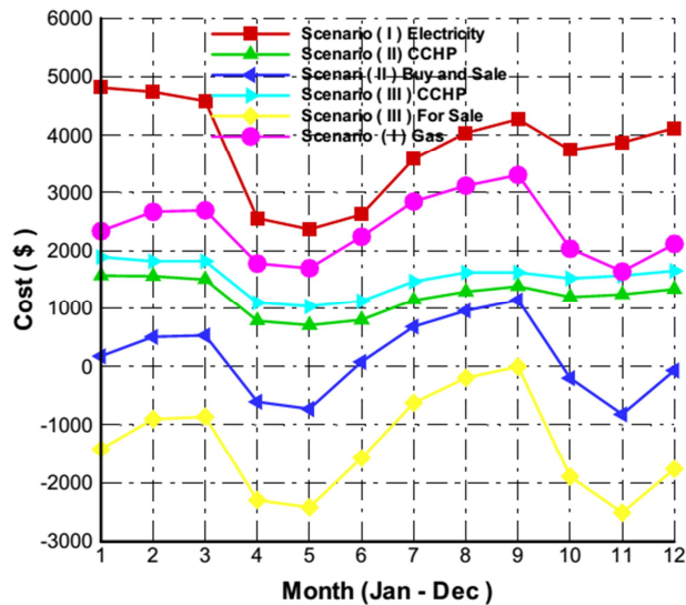
Fig.7 The comparison of the annual costs of defined scenarios
