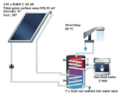
Fig.5 schematic of the DHW supplier cycle
